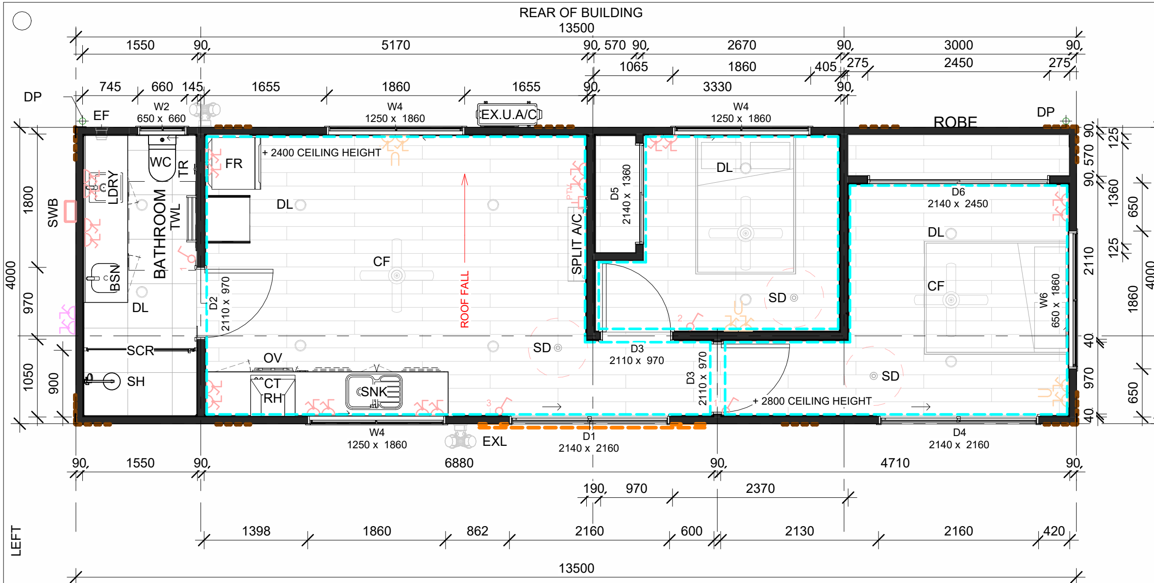
BASE FLOOR PLAN
